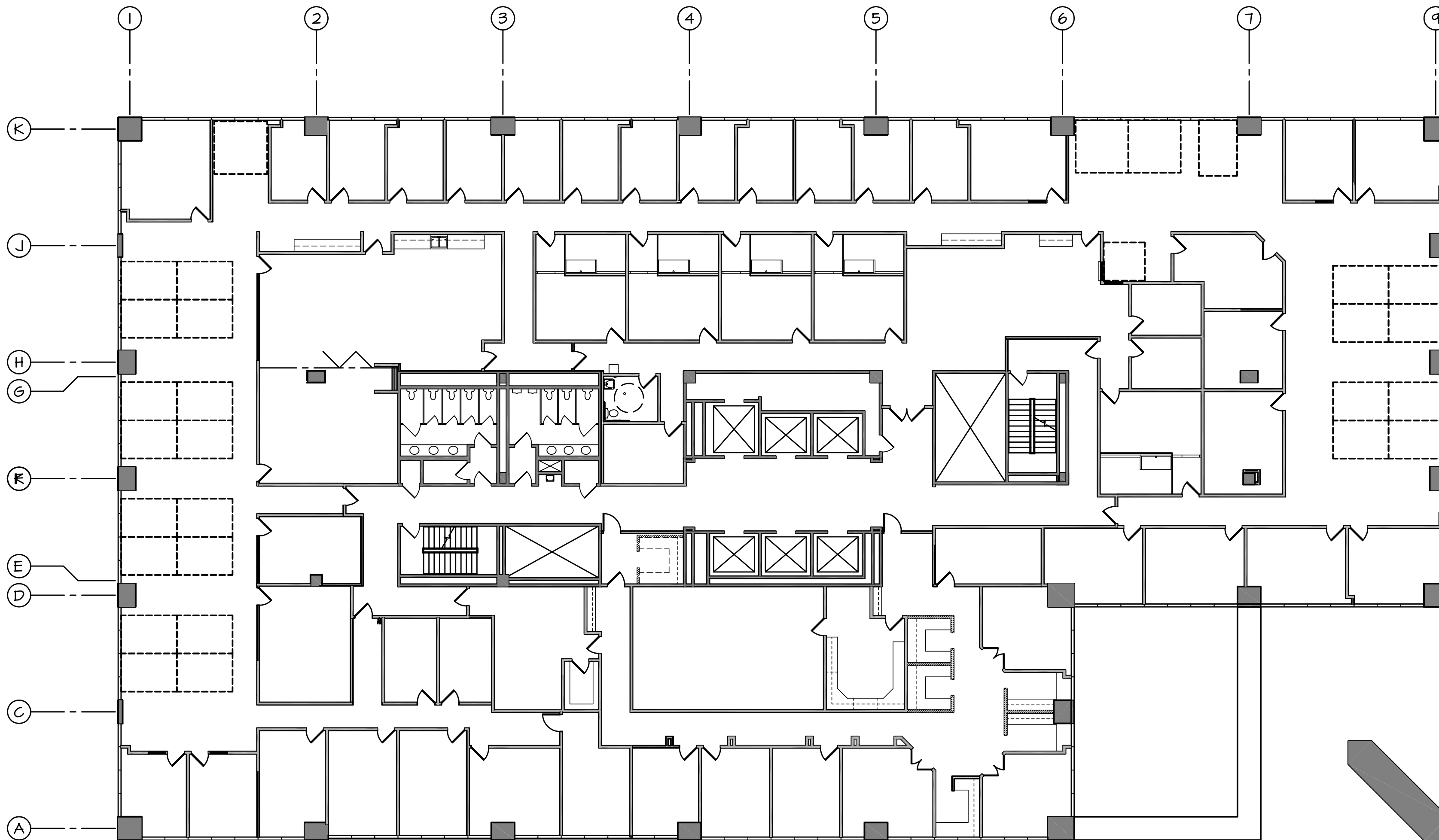
NINTH FLOOR PLAN SCALE: 1/8" = 1'-0"
